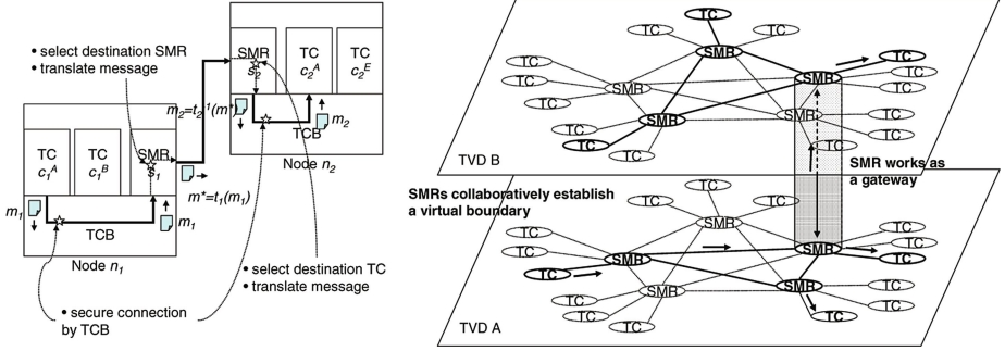
Fig. 5. Multi-domain handling
