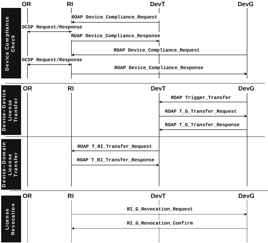
Fig. 3. OMA implementation of transfer
