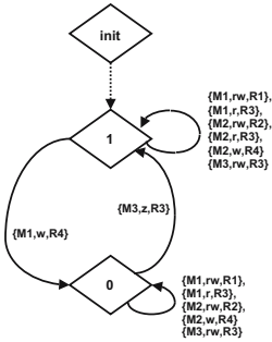
Fig. 4. DFA recognizing legal behavior for a redaction policy
