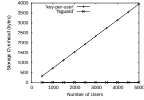
Fig. 2. Storage Overhead
