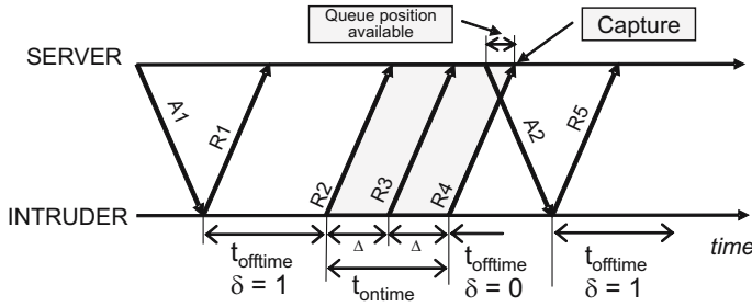
Fig. 5. Attack dynamics
