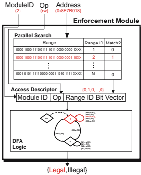
Fig. 3. A hardware reference monitor
